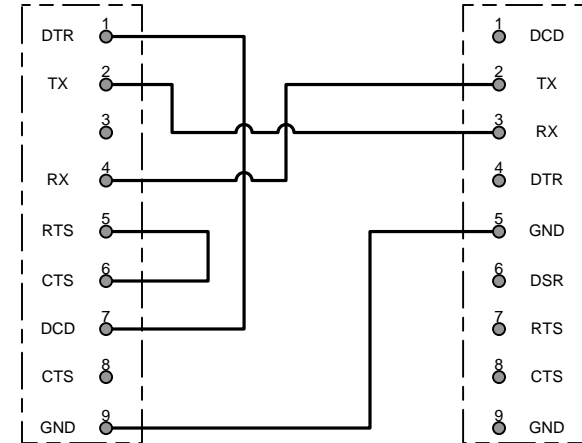
DB-9 MALE CONNECTOR SOLDER CUP (REAR) VIEW
