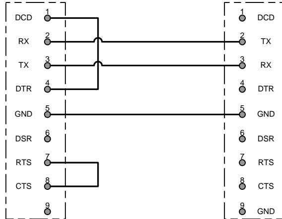
DB-9 FEMALE CONNECTOR SOLDER CUP (REAR) VIEW
